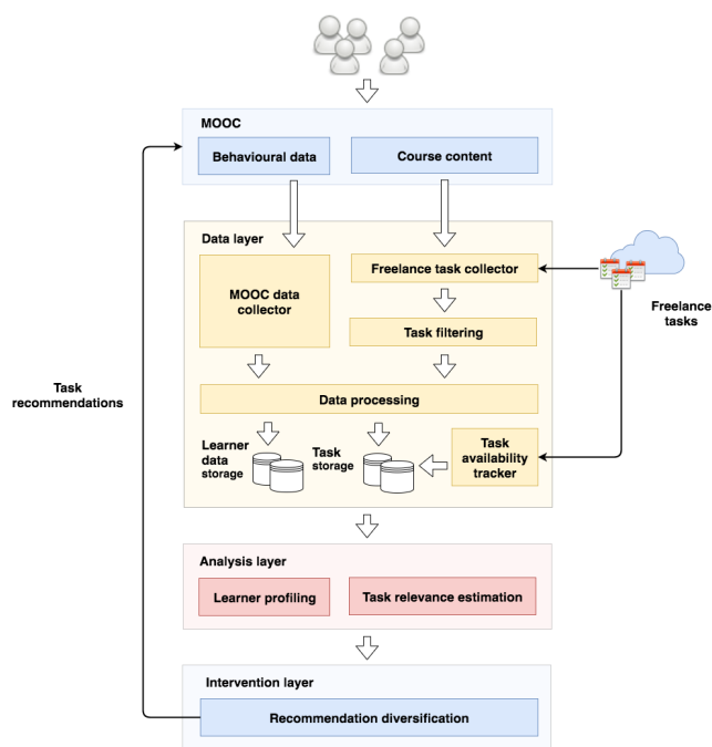
Fig. 7. Overview of the freelance work task recommender system's design.
